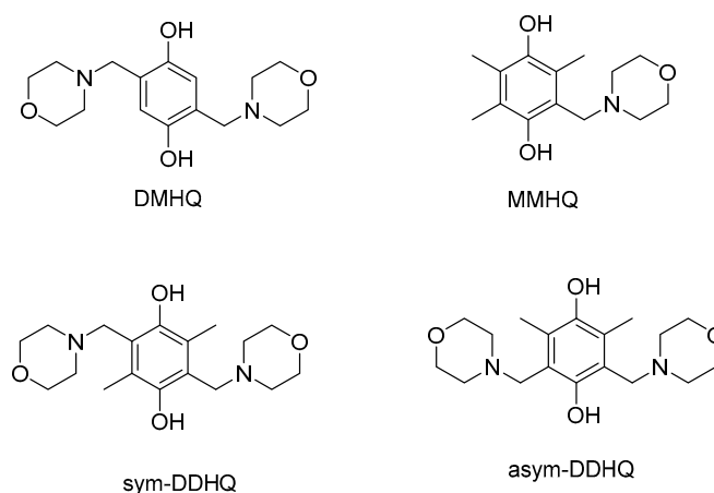
Figure 1. Synthesized Mannich products. IUPAC names of the compounds:
