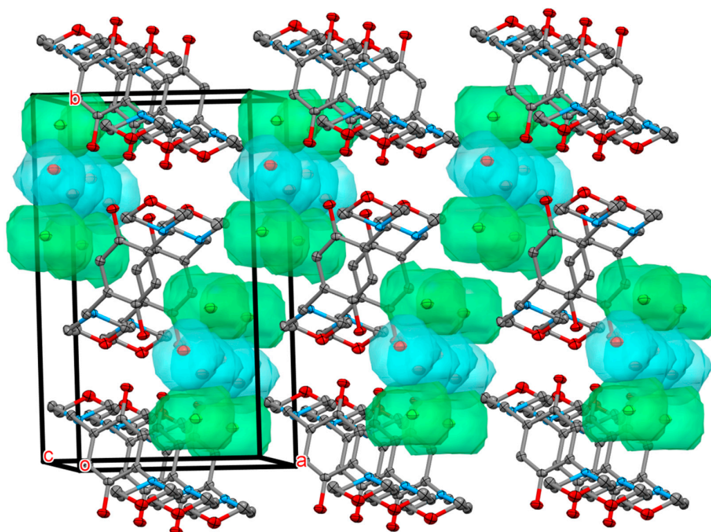
Figure 2. Crystal structure of the hydrochloric salt of DMHQ. Hydrogens are omitted for clarity. Green balls are chloride ions, blue balls are water molecules, and the light green and blue spots show the space available for them in the crystal.
