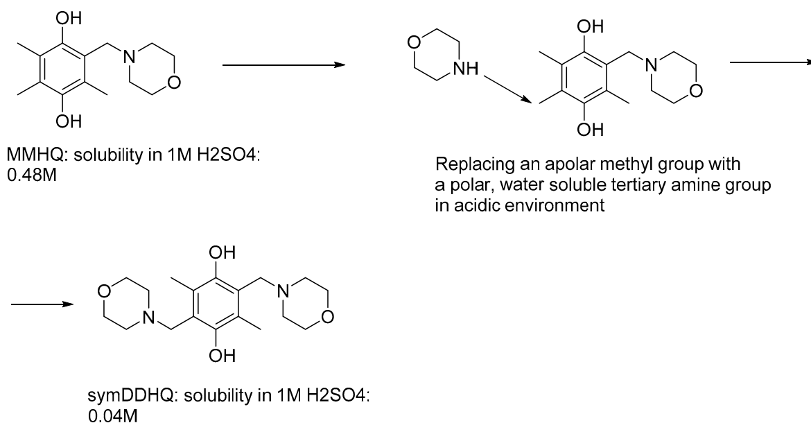
Figure 6. This virtual reaction shows how strongly the molecular symmetry can influence the solubility.
