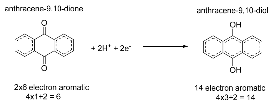
Figure 4. Aromaticity of the anthraquinone/dihydro-anthraquinone redox pair according to Hückel's rule.
