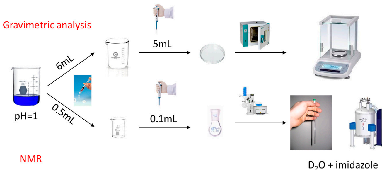
Figure 3. Flow chart of the gravimetric and NMR methods used for determining solubility.
